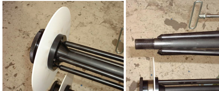
1 or 2 collapsible mandrels.
