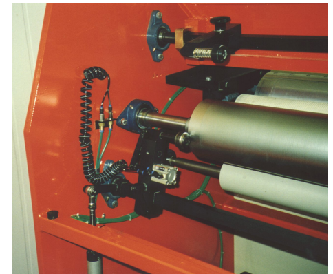
Front arm air assisted collets.
