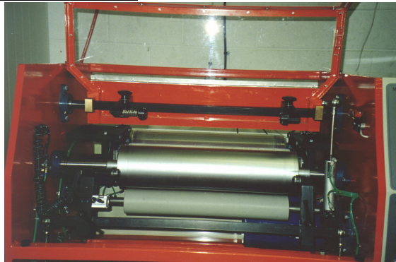
Top arm station for slitting.
